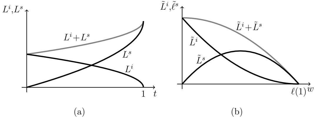
Figure 2: In (a) we depict the contribution of each state of the word t to the imprecision loss L^i(t) \equiv g(\ell'(t)^{-1}) f(t) and the speaking loss L^s(t) \equiv c(\ell(t)) f(t) when g(x) = x , c(w) = w and f \equiv 1 . In (b) we depict the contribution of each word w \in W to the imprecision loss \tilde{L}^i(w) \equiv L^i(\tau(w)) f_\ell(w) and the speaking loss \tilde{L}^s(w) \equiv L^s(\tau(w)) f_\ell(w) .
