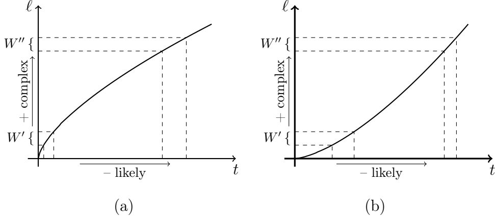
Figure 1: Two examples of a language. In both cases, simple words refer to likely states. In (a) simple words are more precise than complex words, and the contrary is true in (b). See the relative sizes anti-images of the sets W' and W'' , which are of the same size. 9 Note that, when \ell is differentiable, the precision with which a state is communicated is 1_\ell(\ell(t))^{-1} = \ell'(t) .
