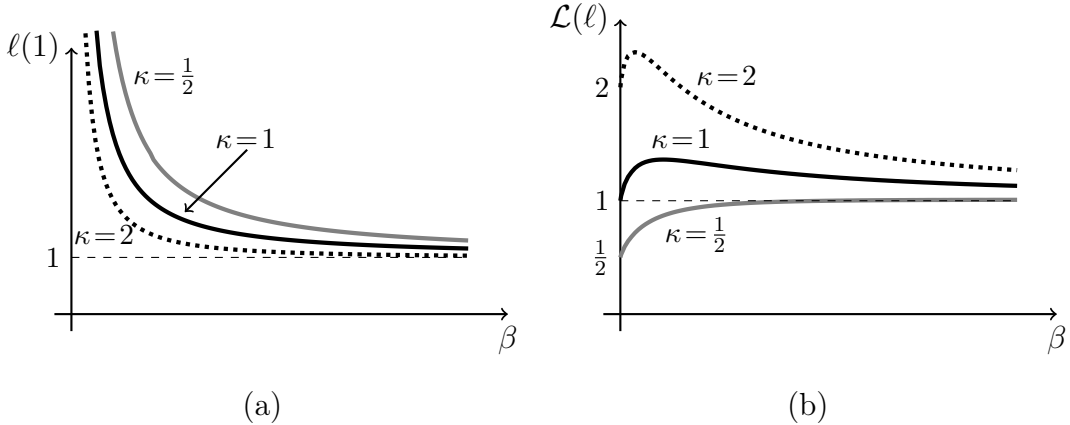
Figure 3: In (a) we depict the optimal vocabulary size \ell(1) as a function of \beta when c(w) = \kappa w^\beta , g(x) = x and f \equiv 1 , for different values of \kappa ; and in (b) we depict the corresponding communication losses. When \kappa is small, the cost of using each word is small too, so the size of the vocabulary is large and the communication loss is low. Similarly, when \beta \rightarrow 0 , we have that c(w) \rightarrow \kappa for all w \in \mathbb{R}_+ , so \ell(1) \rightarrow \infty (the precision of communication increases and the imprecision loss vanishes) and \mathcal{L}(\ell) \rightarrow \kappa . When, instead, \beta \rightarrow \infty , we have that c(w) \rightarrow 0 when w \in [0, 1) and c(w) \rightarrow \infty when w > 1 . As a result, in this case, \ell(1) \rightarrow 1 (and all words have the same precision) and \mathcal{L}(\ell) \rightarrow 1 (the speaking loss vanishes).
